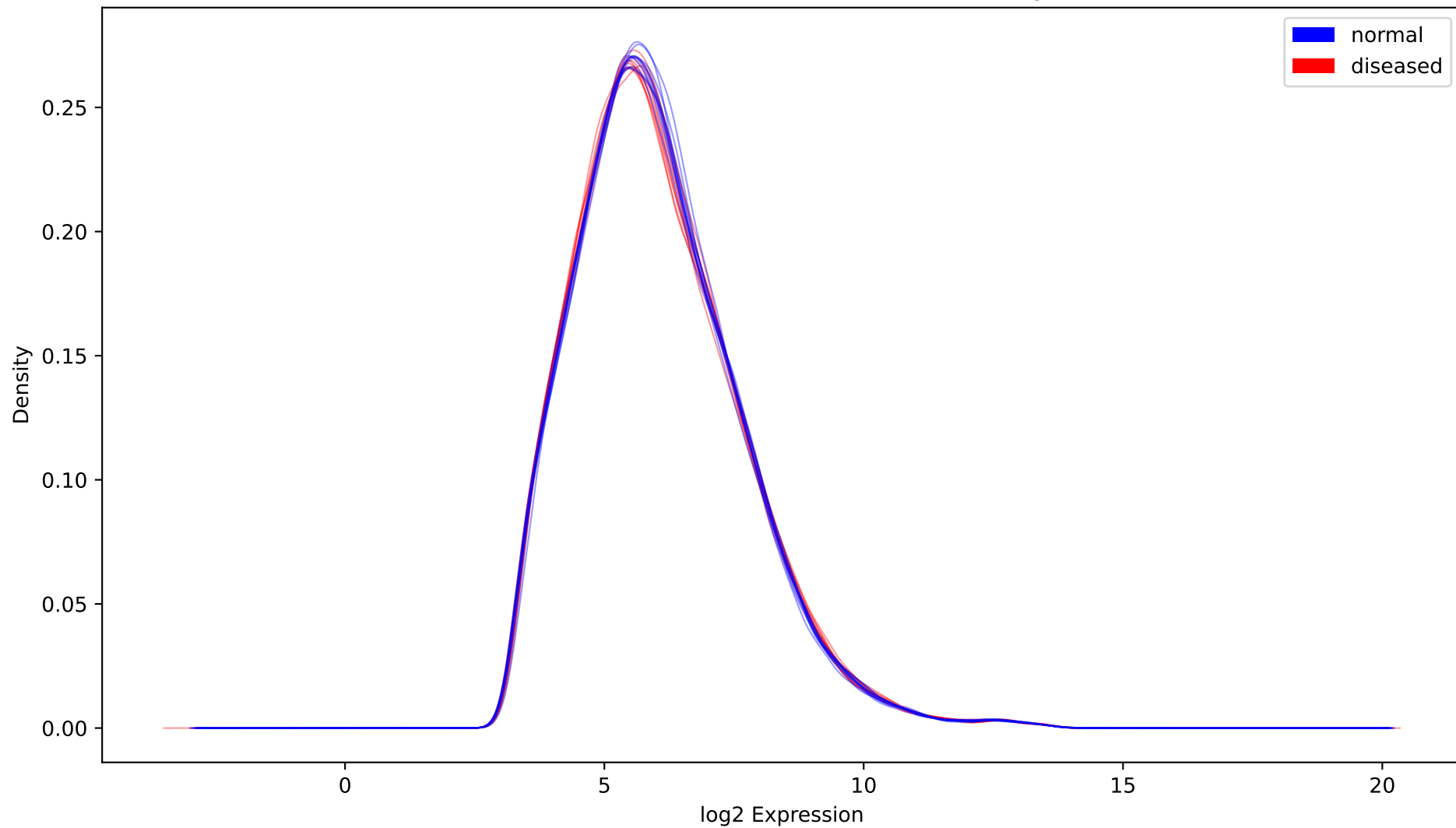
GSE7305: Endometriosis Dataset - Density
